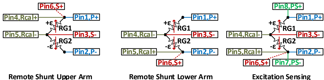
Figure 1-17: Half Bridge Connection for Shunt Calibration (S+ connection is optional)
