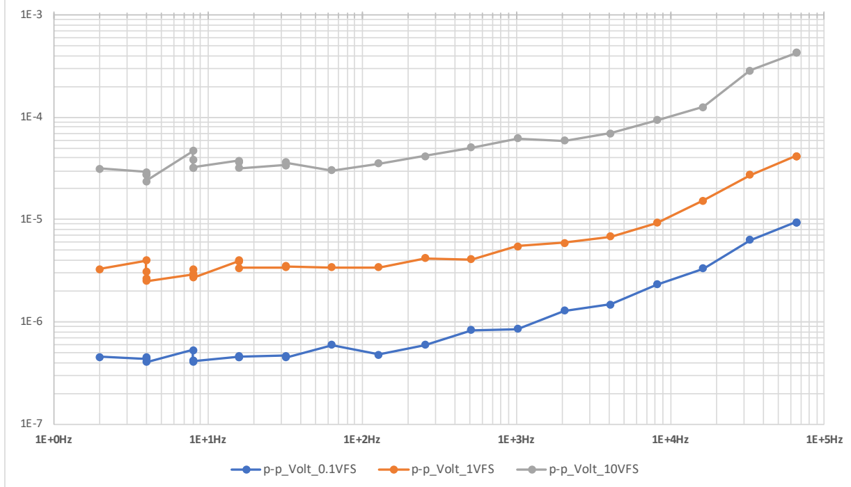
Figure 1-3: Typical peak-to-peak Noise (Volts): Function=Voltage, Range=0.1V, 1V, & 10V
