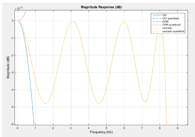
Figure B-8: -EVEN further Zoomed CIC/CFIR Response
