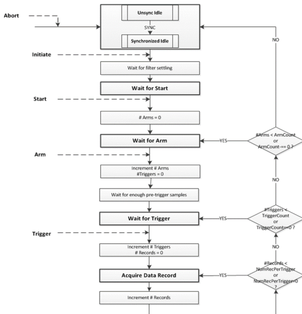
Figure 5-1 Trigger Model
