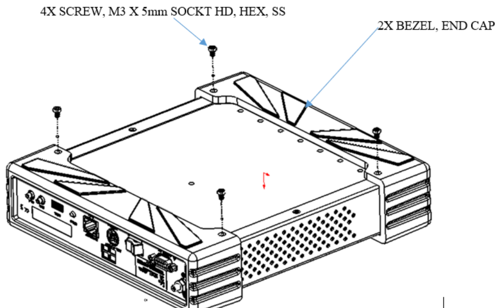
Figure 2-3: TABLETOP Feet Installation Diagram
