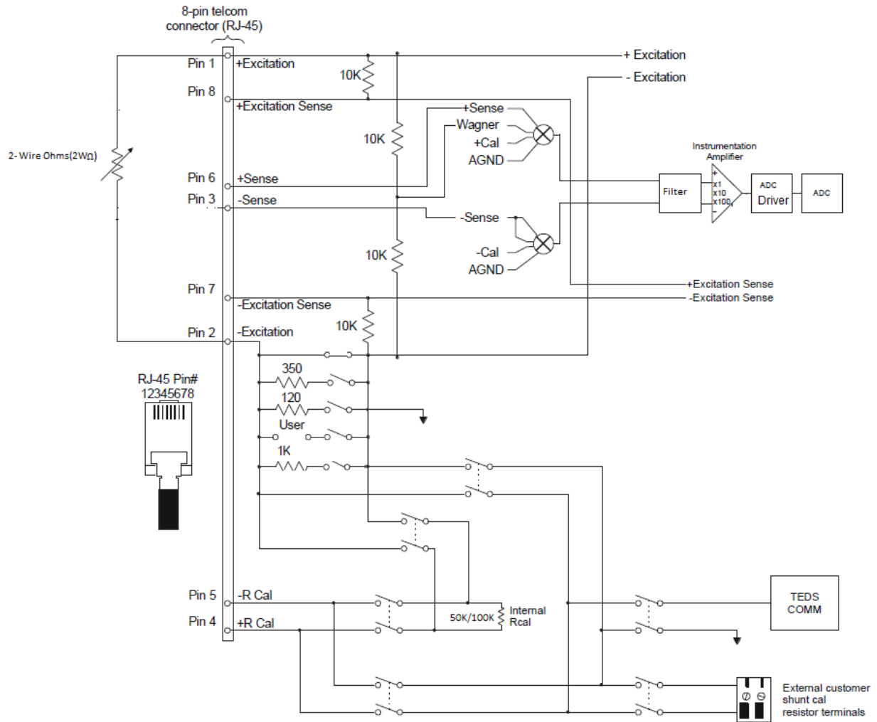
Figure 1-10: Transducer Connection: 2-Wire Ohms (2WΩ)
