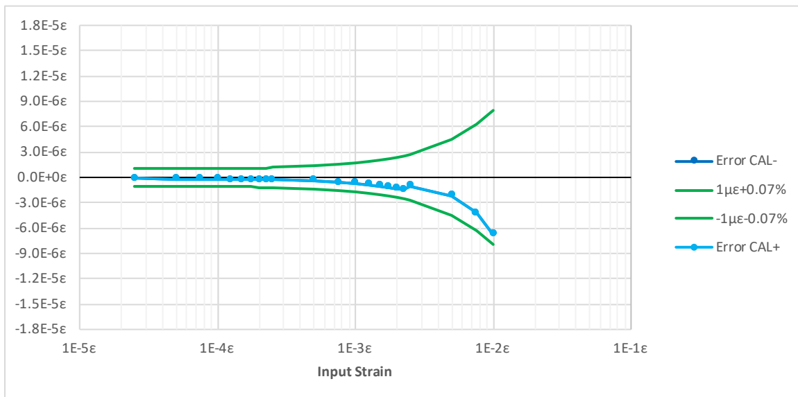
Figure 1-19: FULL BRIDGE Strain Error After Remote Shunt Calibration
