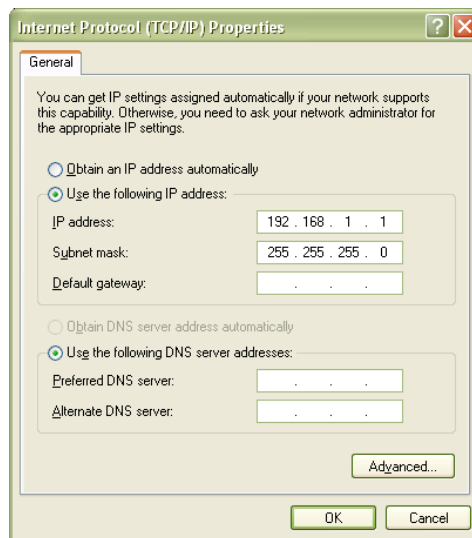
Figure 2-11: Completed NIC Static IP Configuration
