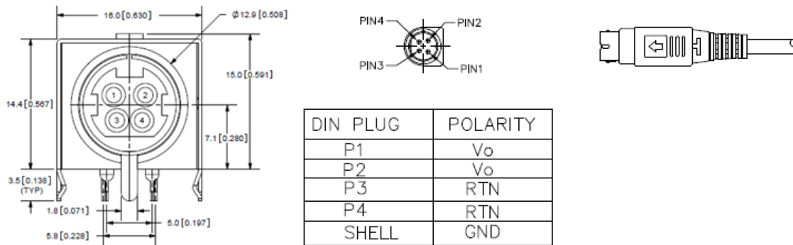
Figure 1-2:: Power Connector Receptacle &amp; Plug
