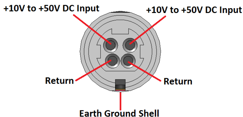
Figure 2-5: Aux DC In connector Pinout
