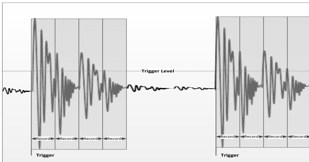
Figure 5-10: Record Size and NumRecordsPerTrigger
