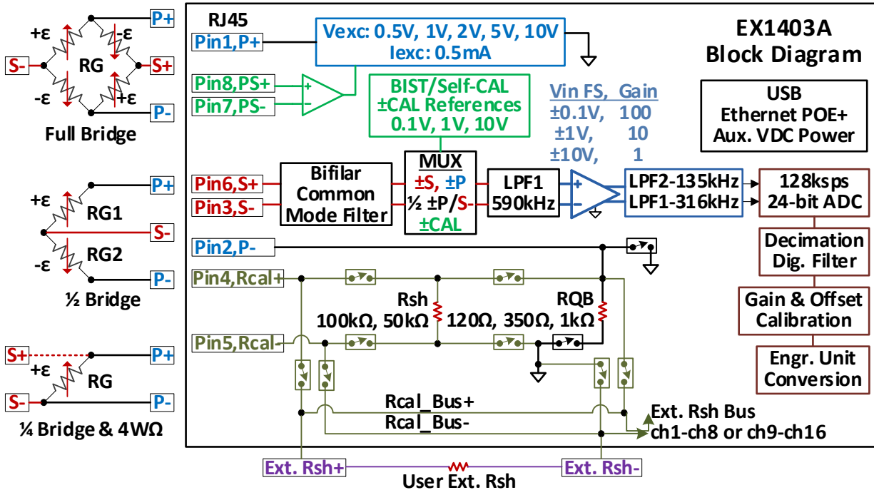
Figure 1-13: Shunt Connection Block Diagram
