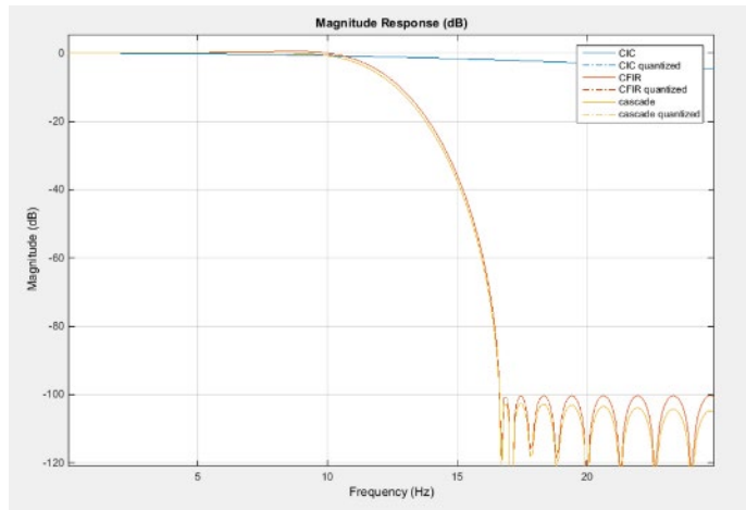
Figure B-7: - further Zoomed CIC/CFIR Response
