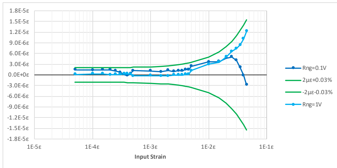
Figure 1-16: QUARTER BRIDGE Strain Error After Remote Shunt Calibration
