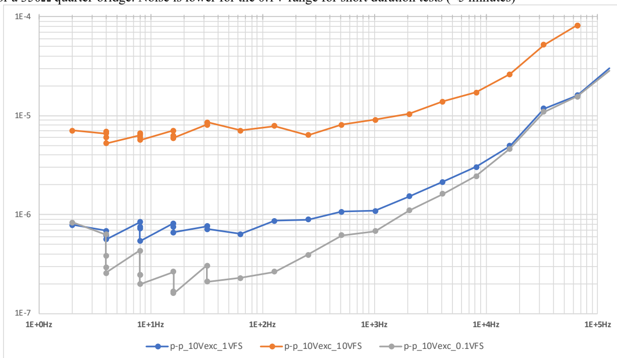
Figure 1-7: Typical peak-to-peak Noise ( \epsilon ): Function=Strain, Range=0.1V, 1V, & 10V
