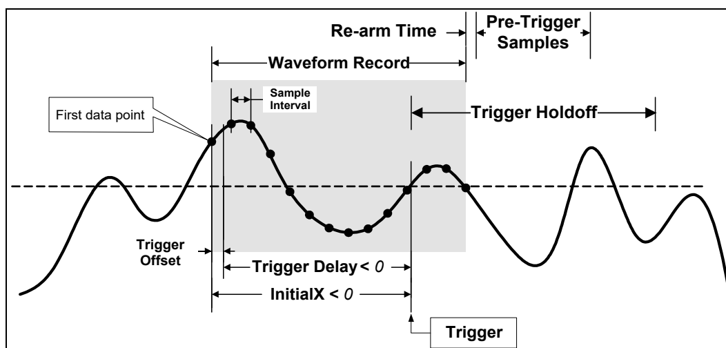
Figure 5-3: Negative Trigger Delay
