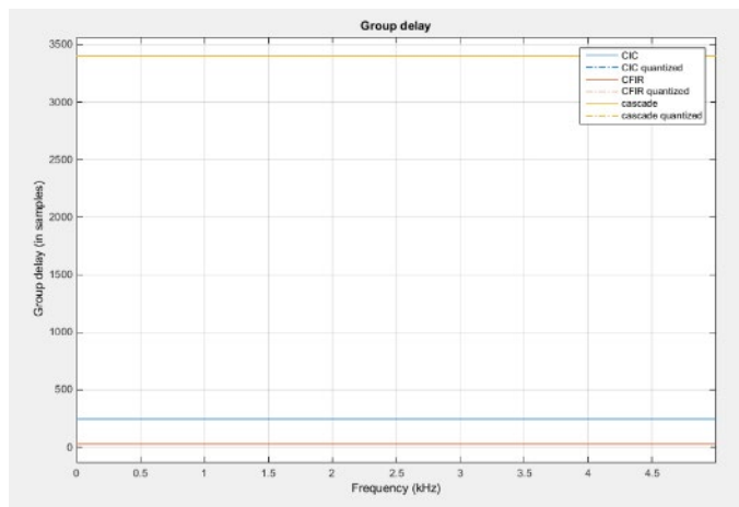
Figure B-5: - CIC/CFIR Group delay
