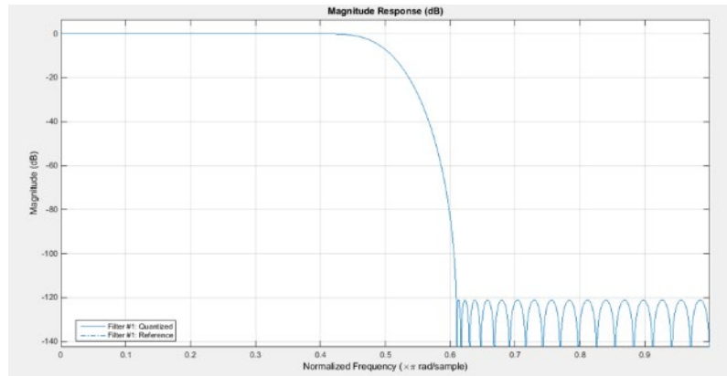
Figure B-2: -: FIR Response
