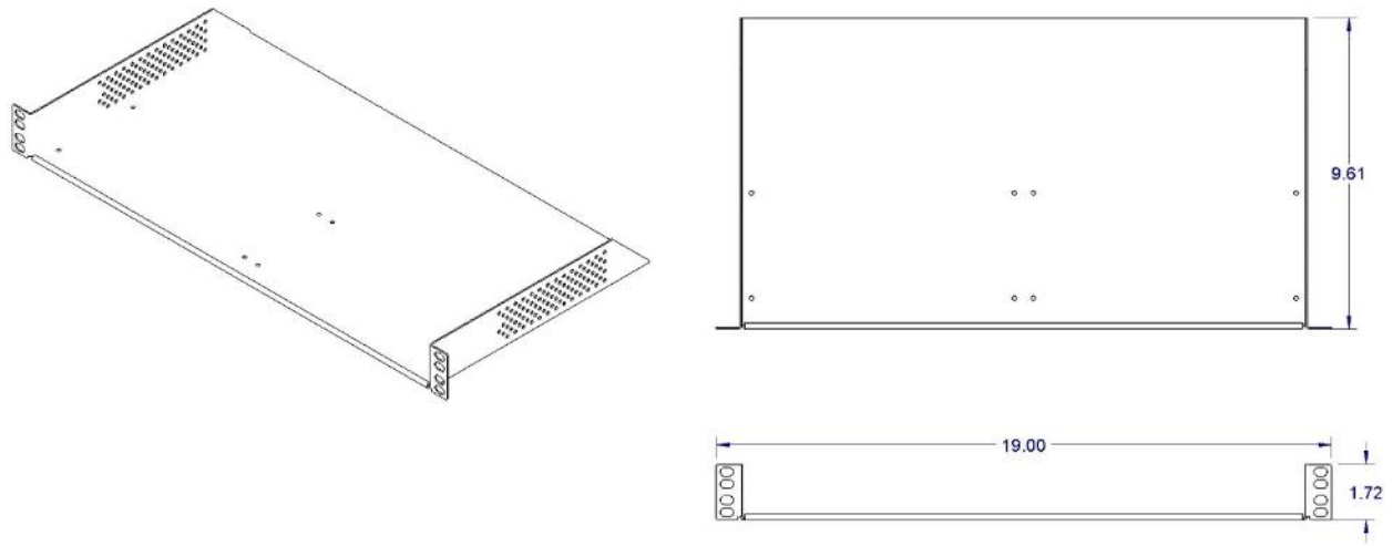
Figure 1-5: EX14XX-RK001RACK MOUNT KIT (inches)
