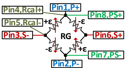
Figure 1-20: Full Bridge Connection for Shunt Calibration
