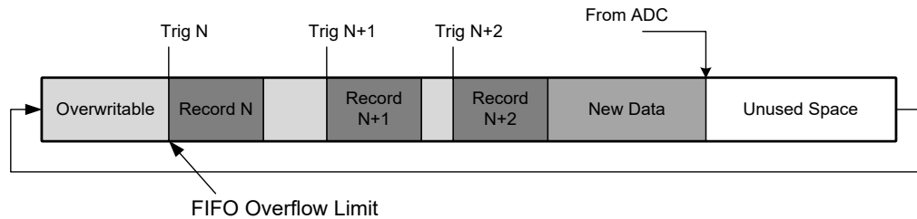
Figure 5-9: Circular FIFO
