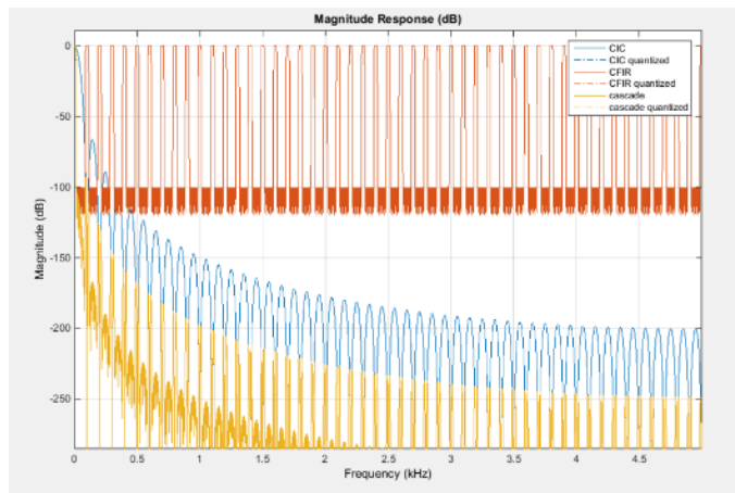
Figure B-4: - CIC/CFIR Filter response up to ADC Nyquist
