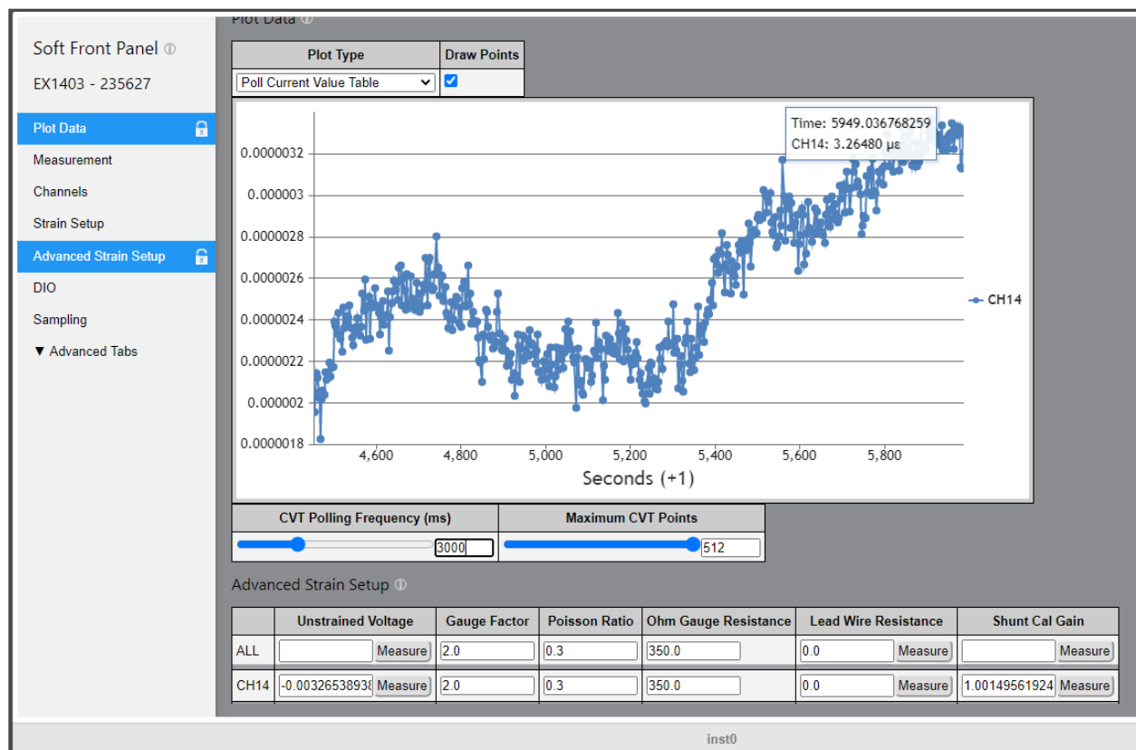
Figure 1-14: Soft Front Panel – Advanced Strain Setup Window
