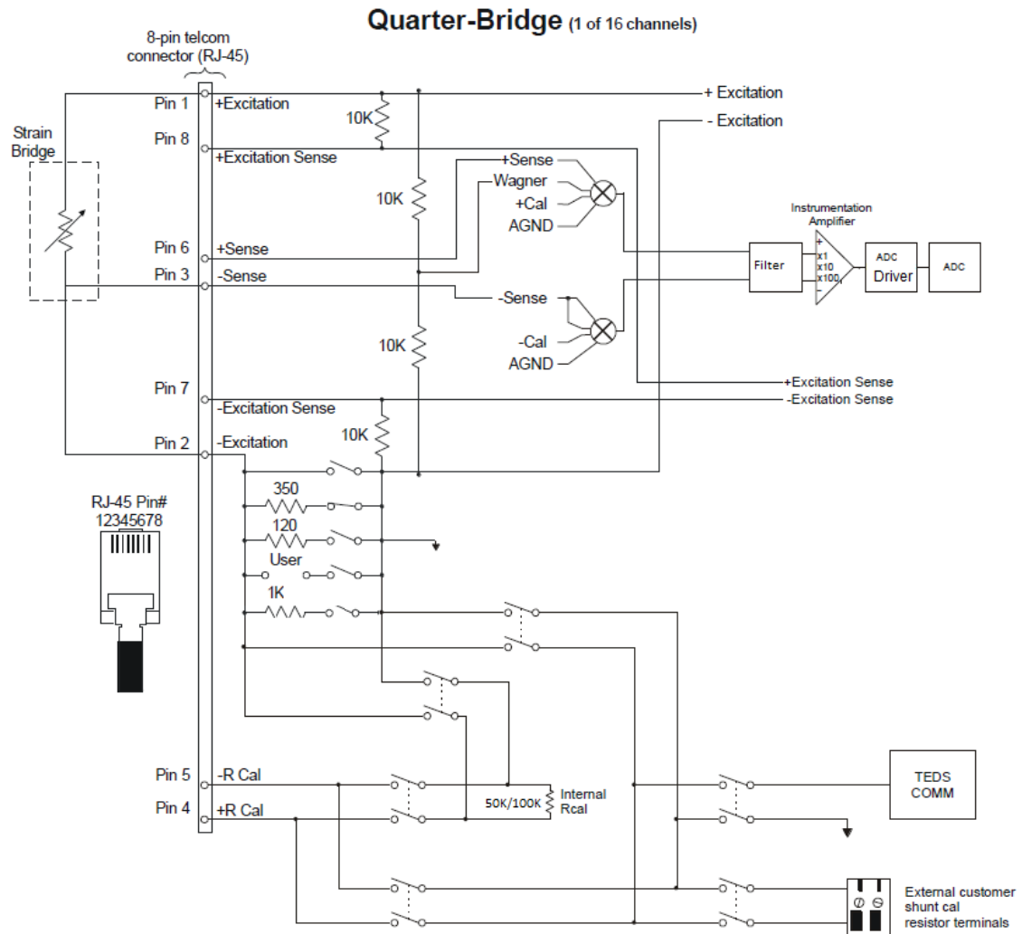
Figure 1-12: teds interface
