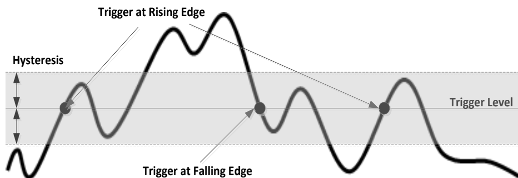
Figure 5-11: Triggering by Analog Signal
