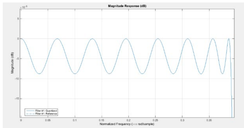
Figure B-3: - Zoomed in to show passband ripple
