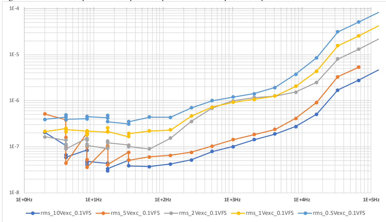
Figure 1-4: Typical RMS Noise ( \epsilon ), Function=Strain, Range=0.1V
