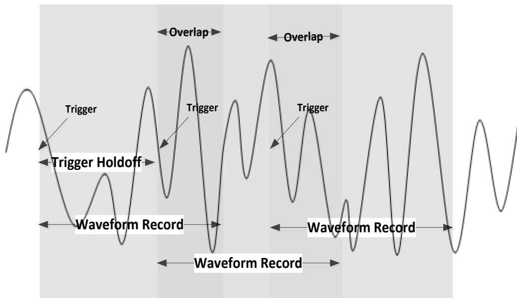
Figure 5-4: Overlapped Data Acquisition
