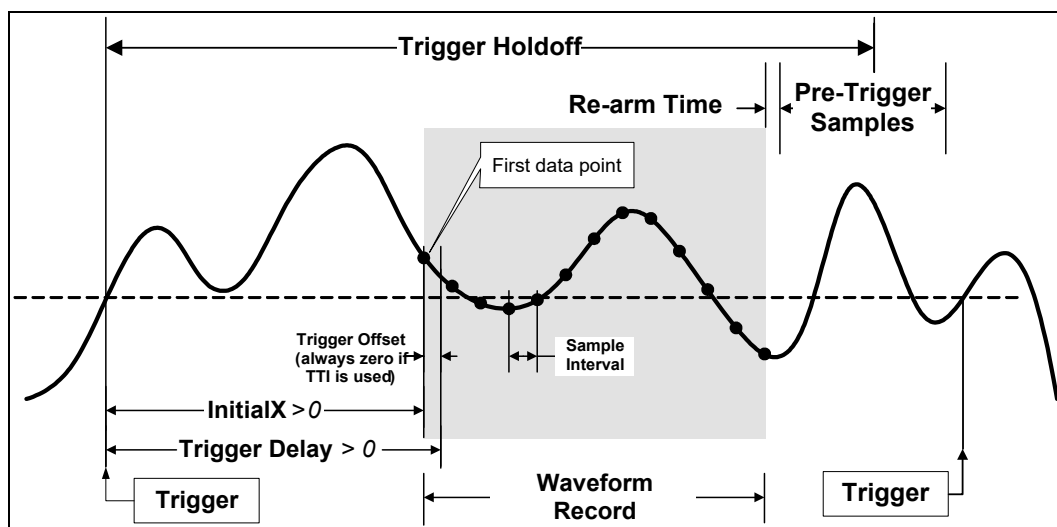
Figure 5-2: Positive Trigger Delay
