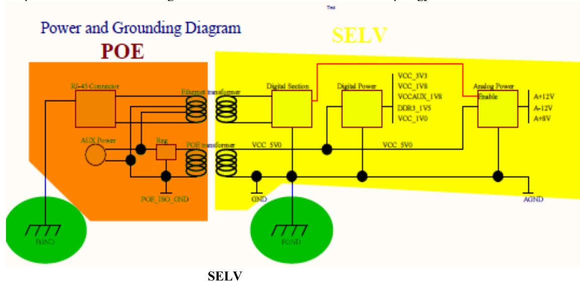
Figure 2-6: EX1403A/EX1403 Power and Grounding
