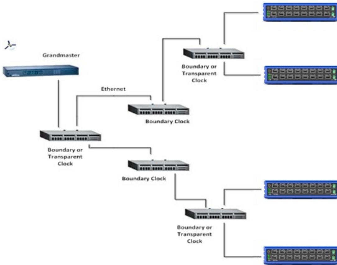
Figure A-1: IEEE1588 Network Topology
