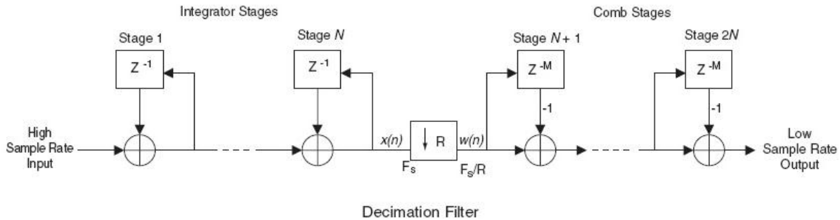
Figure 3.35: CIC Decimation Filter.
