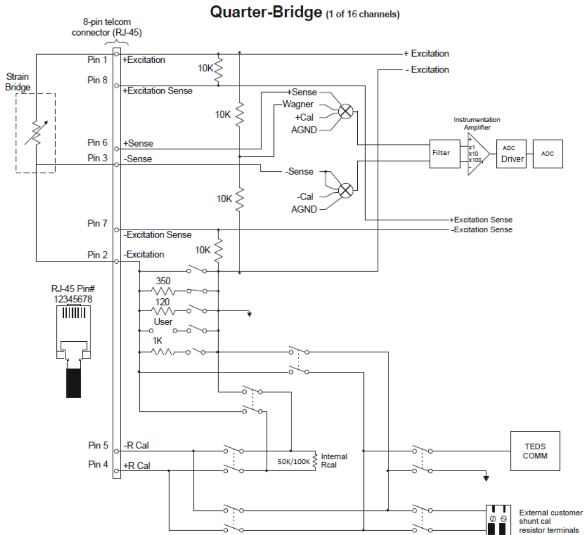
Figure 1-8: Transducer Connection QUARTER BRIDGE with 350 ohm completion
