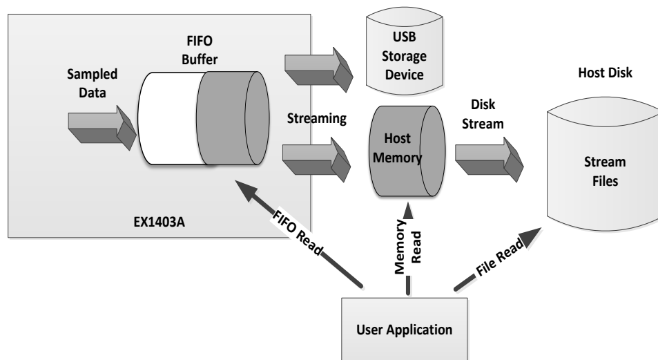
Figure 5-5: FIFO Read and Streaming
