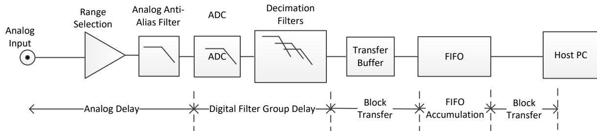
Figure 5-12: Delays in Data Path
