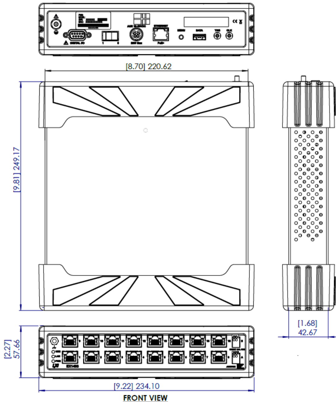
Figure 1-4:: EX1403A/EX1403 Dimensions [inch] mm
