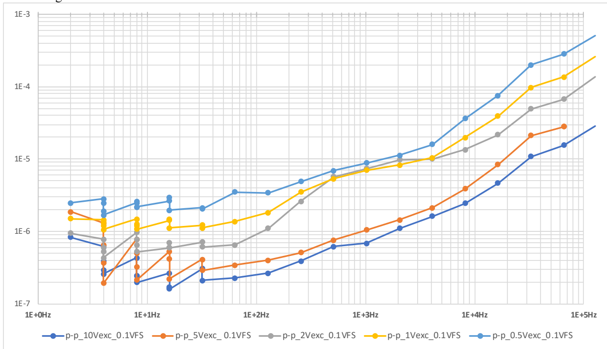
Figure 1-5: Typical peak-to-peak Noise ( \epsilon ), Function= Strain, Range=0.1V
