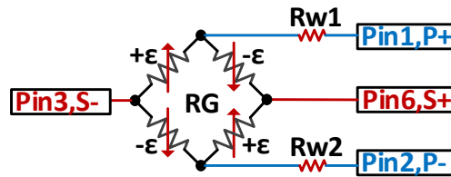
Figure 1-23: Lead Wires for Full Bridge Connection
