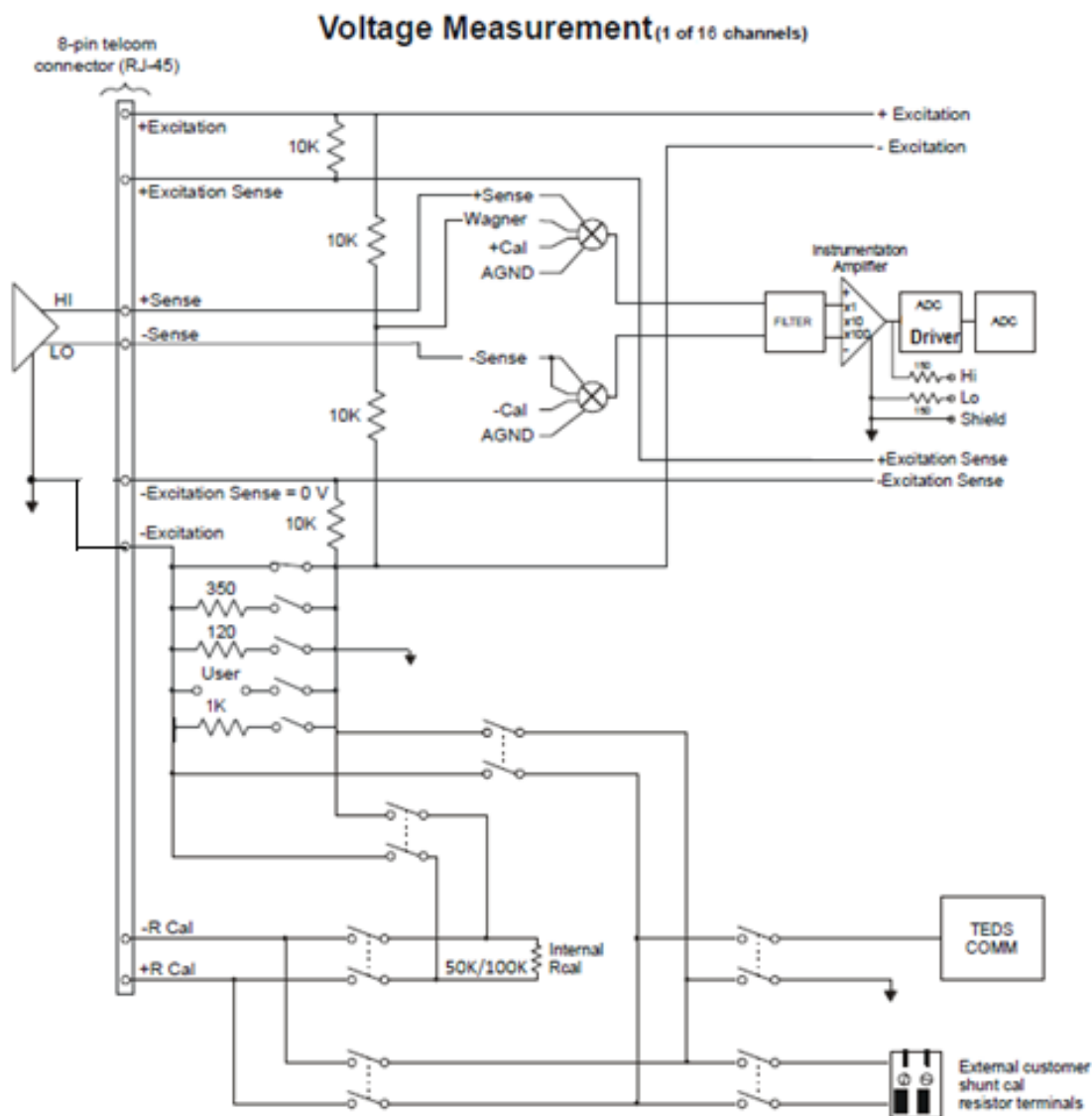
Figure 1-9: VOLTAGE MEASUREMENT CONFIGURATION (DIFFERENTIAL INPUT)
