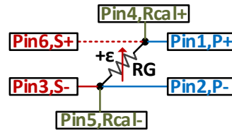
Figure 1-15: Quarter Bridge Connection for Shunt Calibration (S+ connection is optional)
