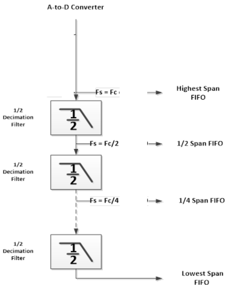
Figure 5-8: Decimation Filter and Measurement Span
