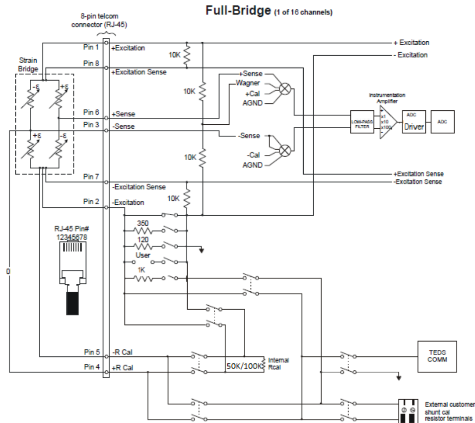
Figure 1-6: Transducer Connection: Full Bridge
