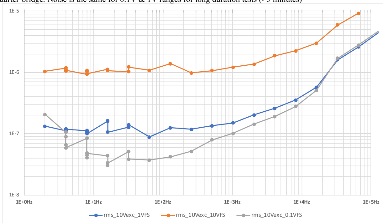
Figure 1-6: Typical RMS Noise ( \epsilon ): Function=Strain, Range=0.1V, 1V, & 10V
