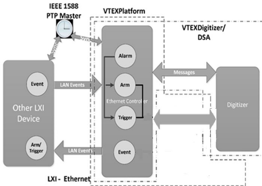
Figure 5-6: LXI and LAN Events
