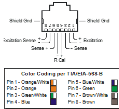
Figure 1-1: RJ-45 Transducer Input Connector Pin Assignment
