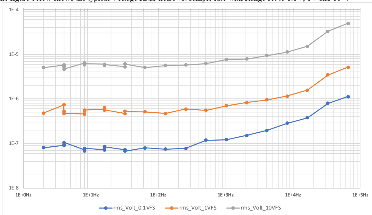
Figure 1-2: Typical RMS Noise (Volts): Function=Voltage, Range=0.1V, 1V, & 10V
