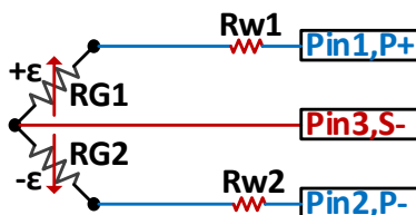
Figure 1-22: Lead Wires for Half Bridge Connection
