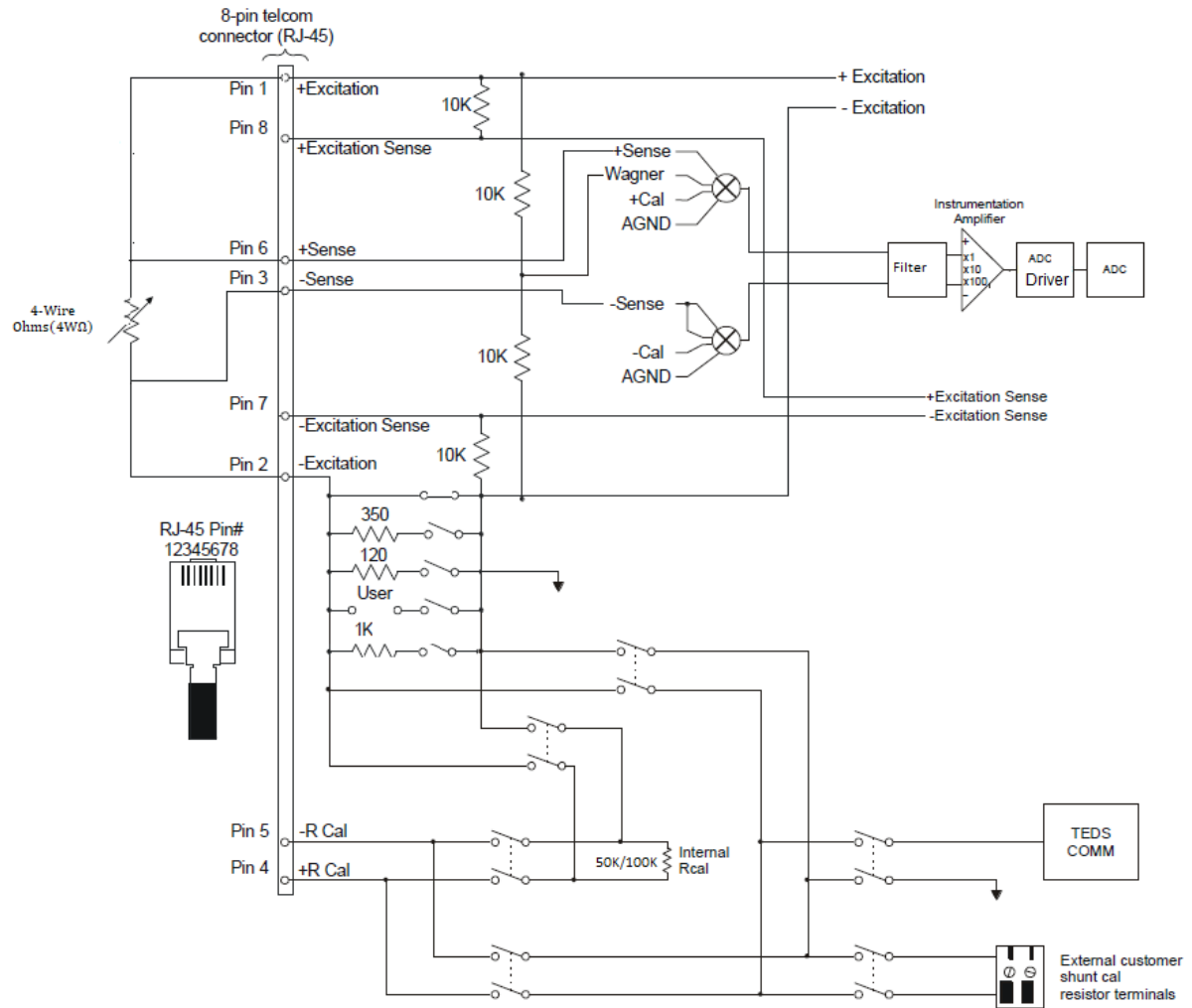
Figure 1-11: Transducer Connection: 4-Wire Ohms (4WΩ)
