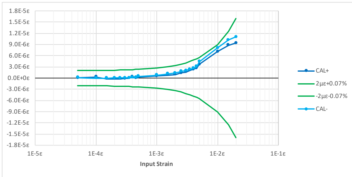
Figure 1-18: HALF BRIDGE Strain Error After Remote Shunt Calibration
