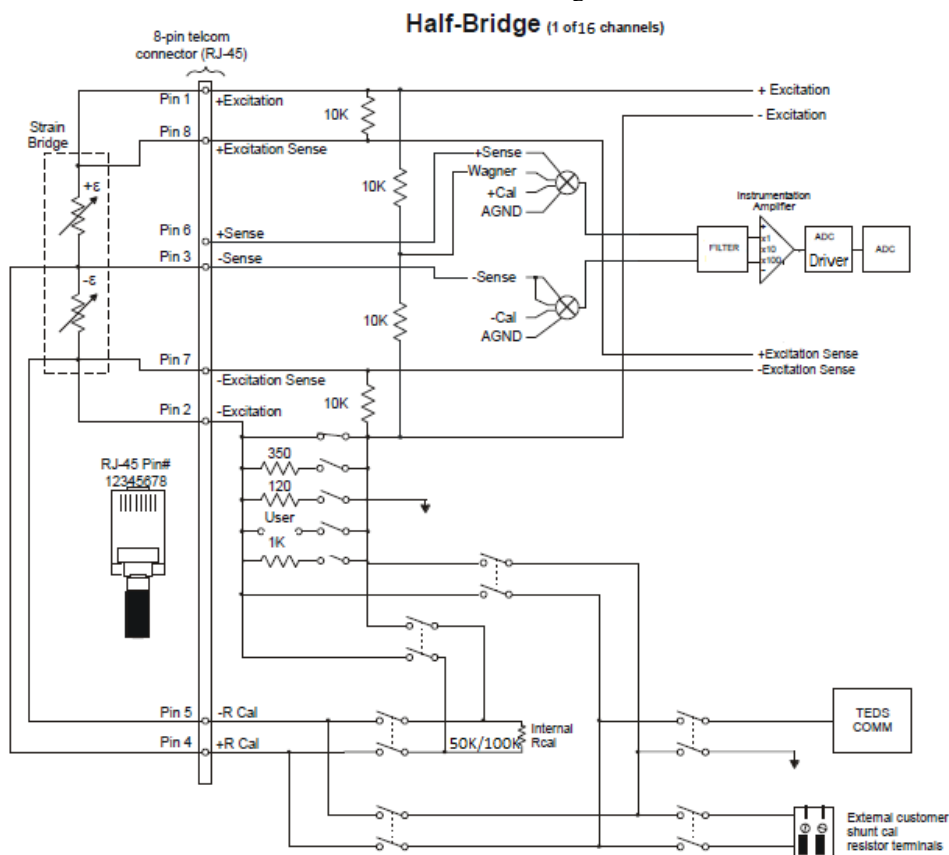
Figure 1-7: Transducer Connection: half Bridge
