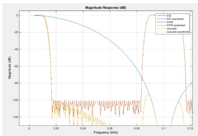
Figure B-6: - Zoomed CIC/CFIR Response
