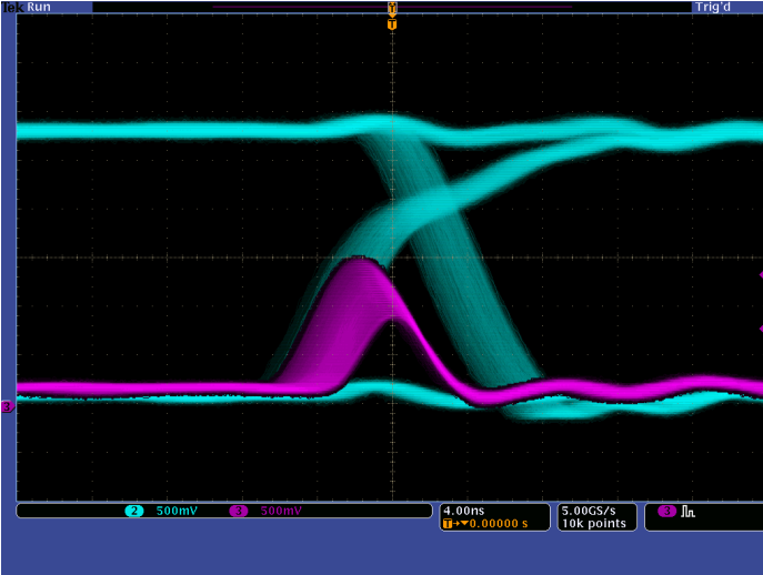
Digital phosphor technology enables greater than 50,000 wfms/s waveform capture rate and real-time intensity grading on the MSO/DPO4000 Series.
