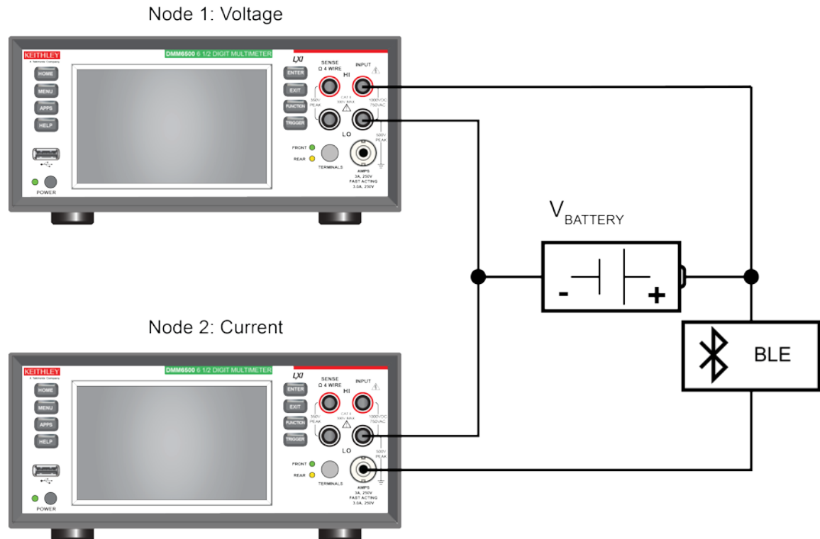
Figure 43: Two nodes measuring current and voltage
