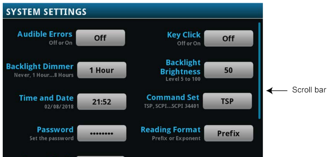
Figure 2: Scroll bar
