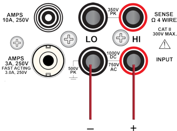
Figure 32: Rear-panel connections
