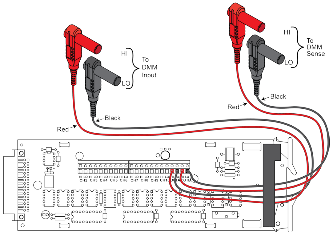
Figure 37: 2001-TCSCAN card
