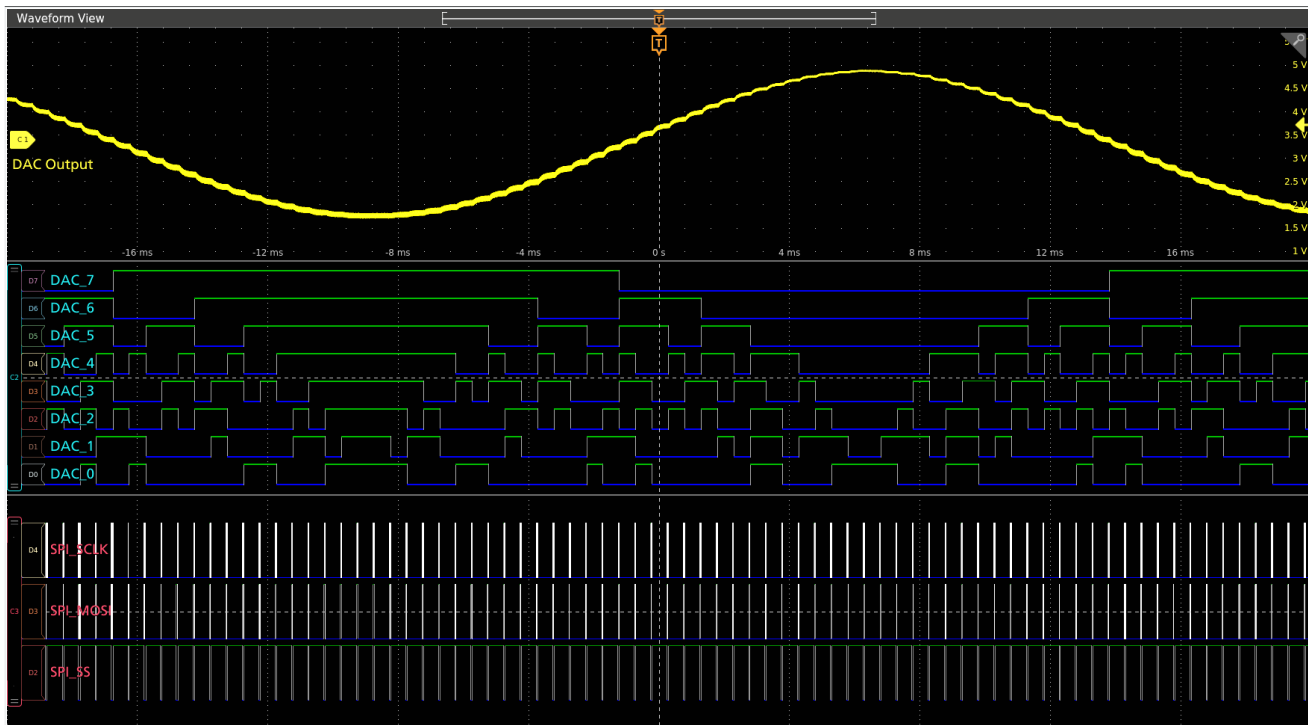
The TLP058 provides eight high performance digital inputs. Connect as many TLP058 probes as you like, enabling up to a maximum of 64 digital channels.
