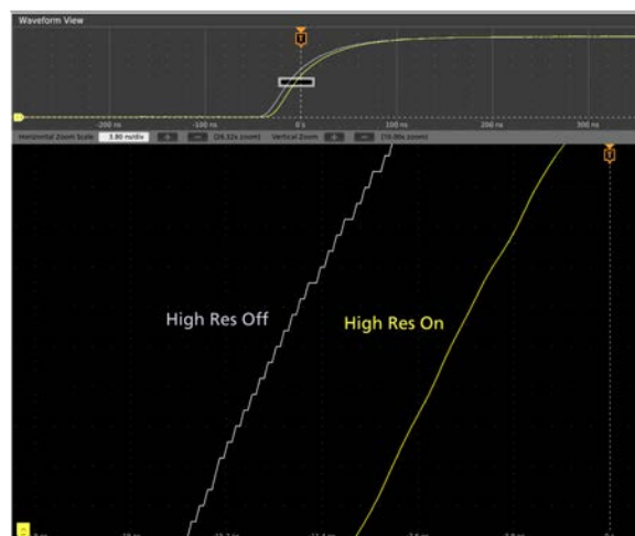
Figure 12: The 6 Series MSO's 12-bit ADC, along with the new High Res mode, enable industry leading vertical resolution.
