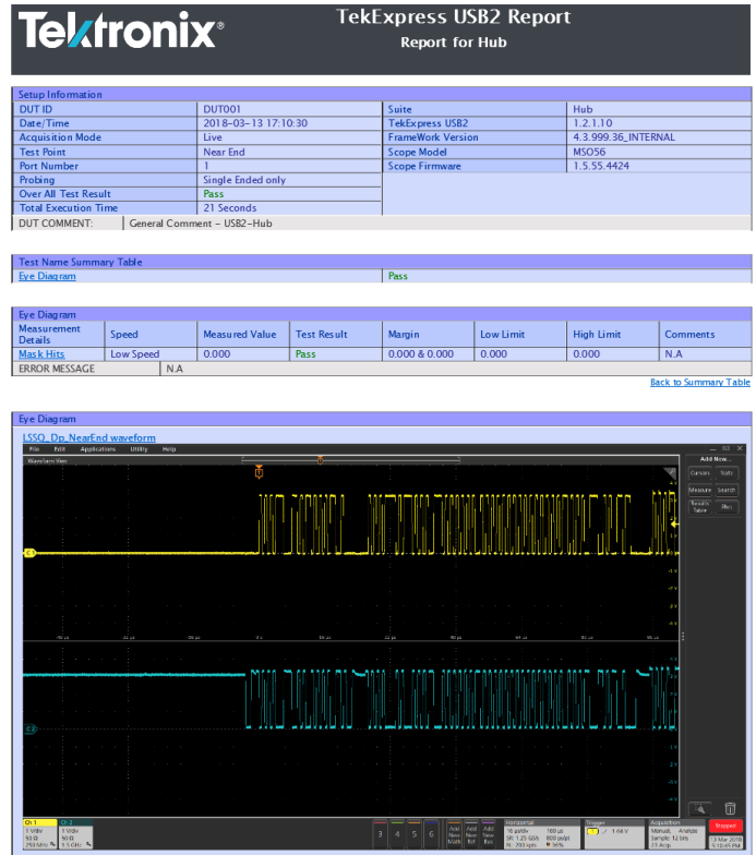
TekExpress USB2 report showing setup details and measurement results
