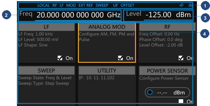
Figure 1-8 User Interface
