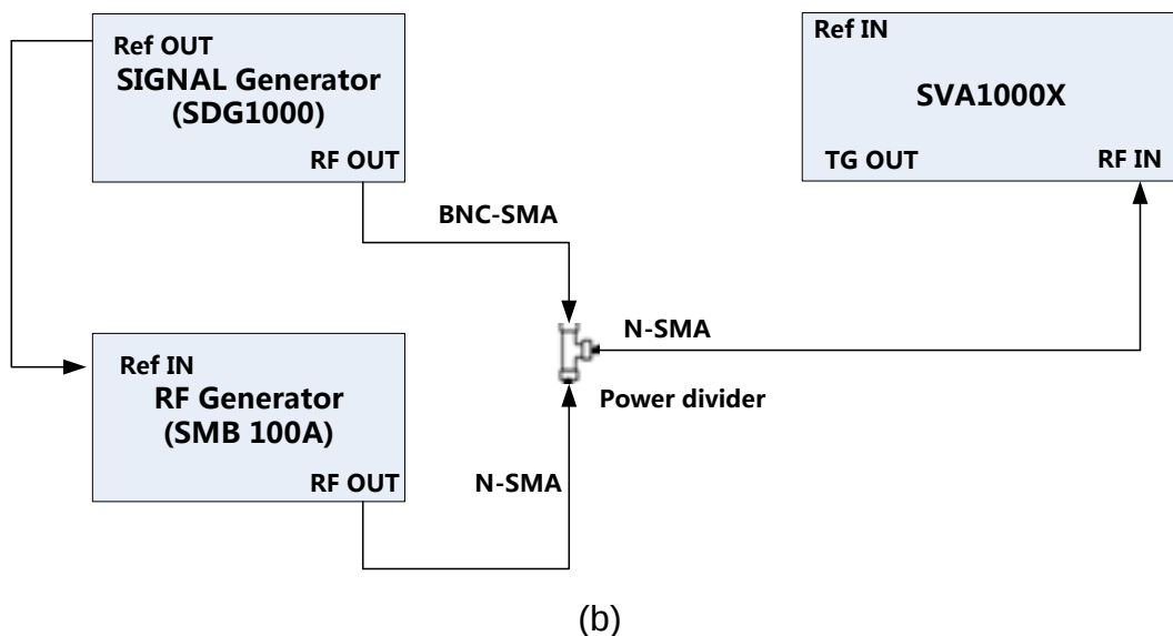
Figure 3-7 connecting test instruments for 1dB Gain Compression Test
