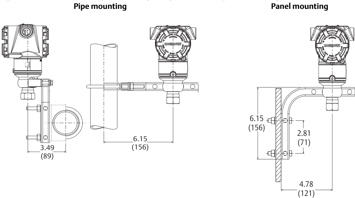
Figure 13. Rosemount 3051T Typical Mounting Configurations with Optional Mounting Bracket
