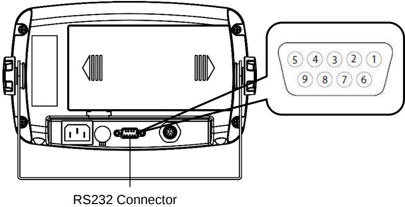
Figure 2-5 i-DT33P RS232 Connector
