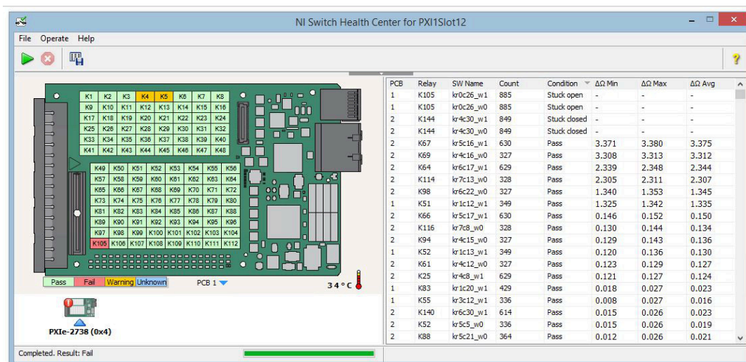
Figure 2. The NI Switch Health center provides advanced relay health monitoring options, including functional and resistive self-tests, onboard relay count tracking, and report generation.
