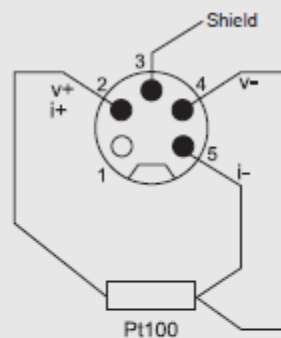
3-wire PRT connection
