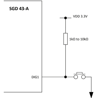
Generating a digital input with a push button
