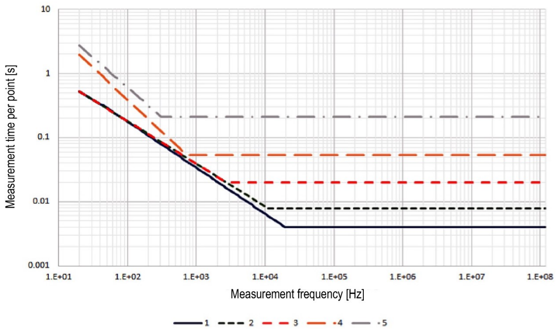
Figure 3. Measurement time (Option 120, adapter: 7 mm 42942A/probe 42941A, Typical)
