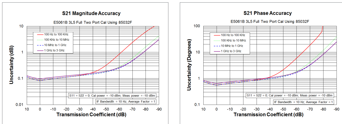
Figure 1. Transmission uncertainty (specification)
