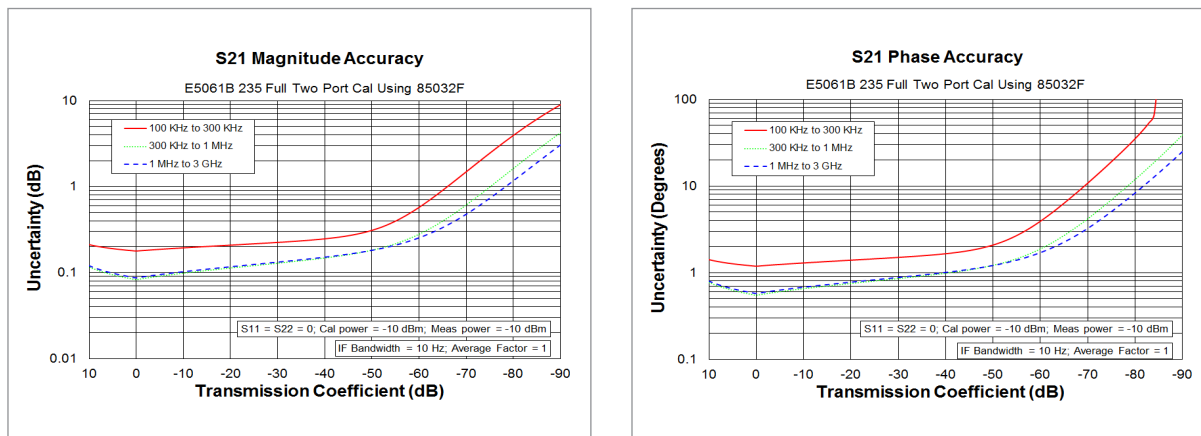
Figure 7. Transmission uncertainty (specification)
