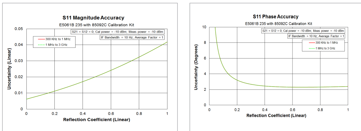
Figure 12. Reflection uncertainty (specification)
