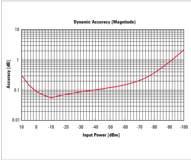
Figure 17. Dynamic Accuracy Option 3L3/3L4/3L5
