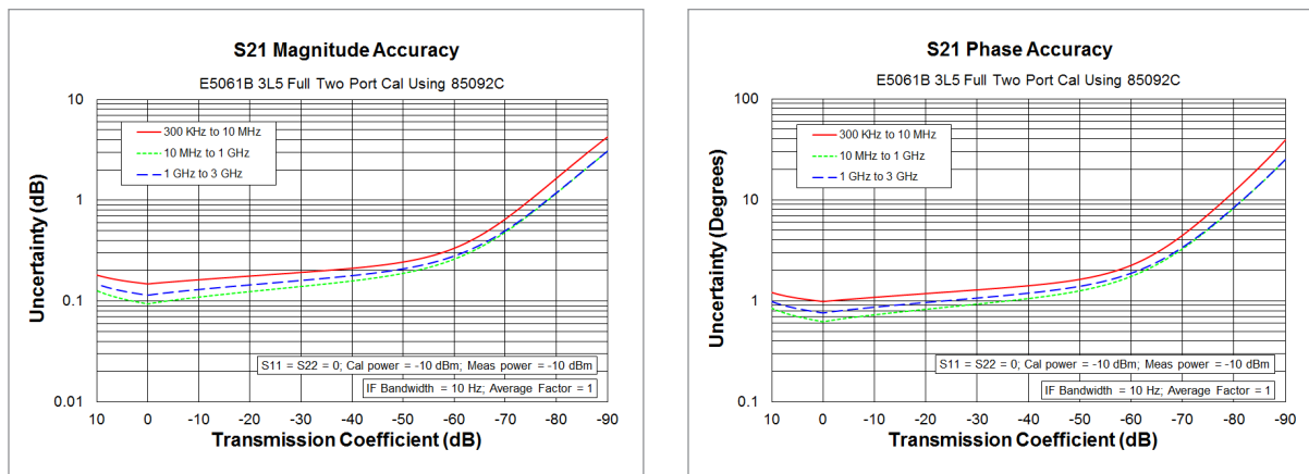
Figure 5. Transmission uncertainty (specification)
