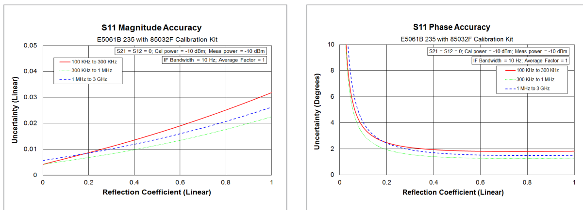
Figure 8. Reflection uncertainty (specification)
