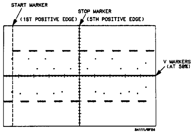
Figure 9-4. Start and Stop on Edges.
