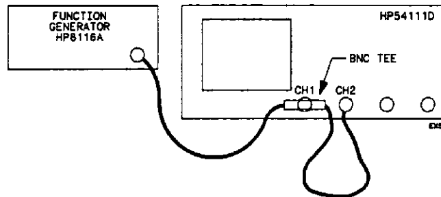
Figure 6-15. Equipment Connection.
