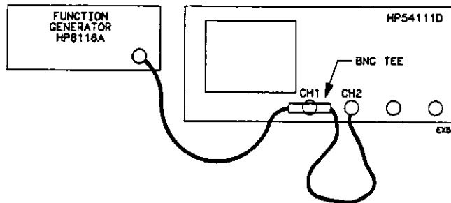
Figure 6-4. Equipment Connection
