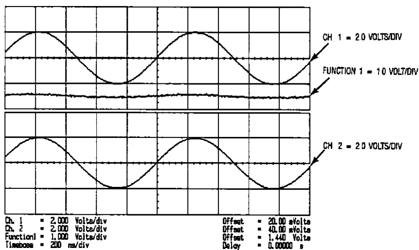
Figure 11-3. Subtracting Two Operands
