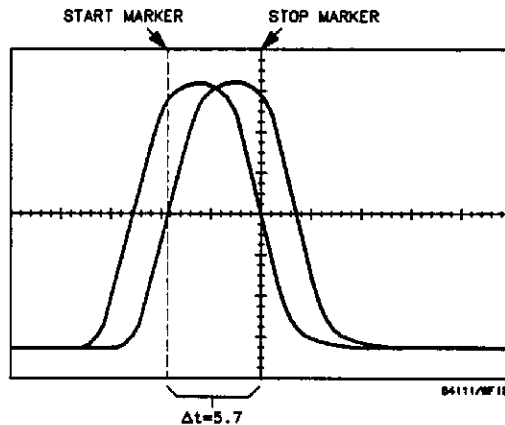
Figure 6-10. Waveform With 5.7 ns Overlap.
