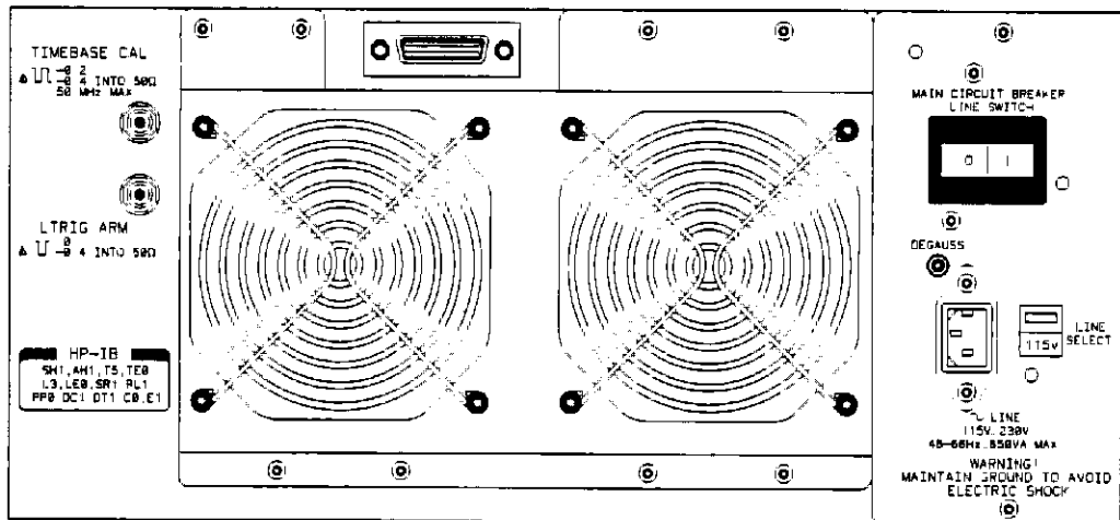
Figure 2-2. 54111D Rear Panel
