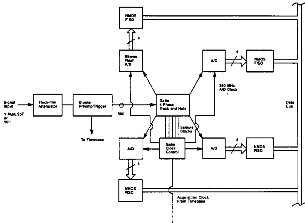
Figure B-1. HP 54111D Signal Acquisition.
