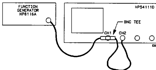
Figure 6-12. Equipment Connection.
