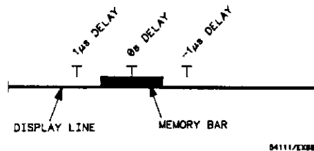
Figure 7-4 Memory Bar With \pm 1 \mu s Delay.
