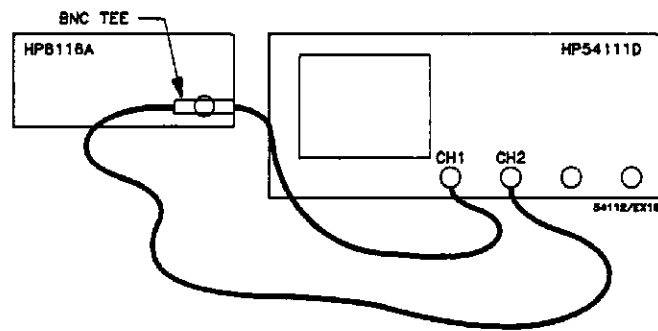
Figure 11-2. Equipment Set-up
