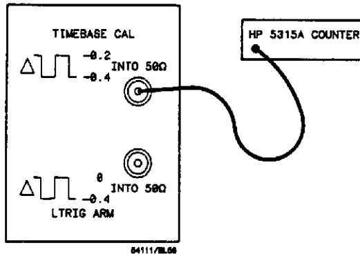
Figure 14-5. Timebase Freq Cal Instrument Setup.
