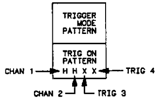
Figure 6-7. Setting the Pattern.
