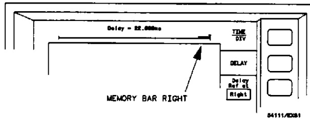
Figure 5-2. Memory Bar at Delay Left/Center/Right.
