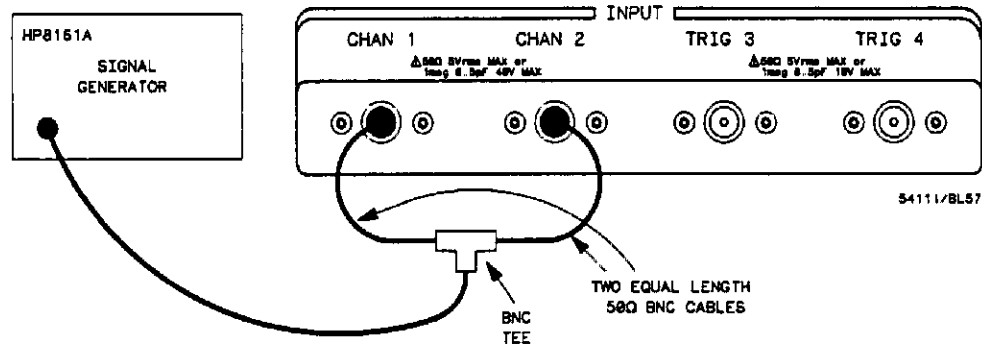
Figure 14-4. Channel Skew Instrument Setup.
