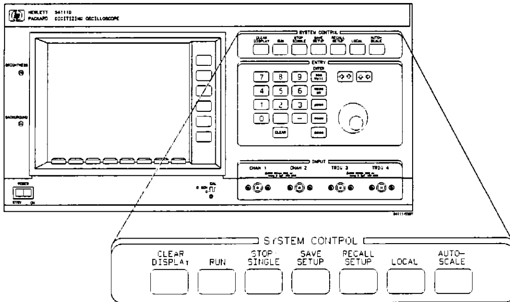
Figure 3-1. System Control Keys.
