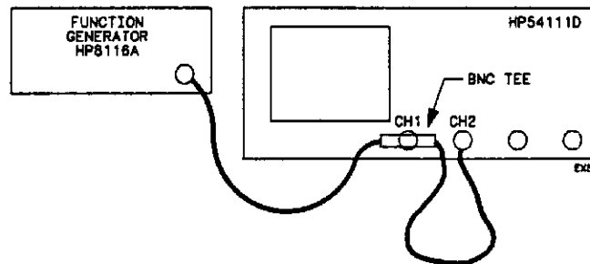
Figure 6-17. Equipment Connection.
