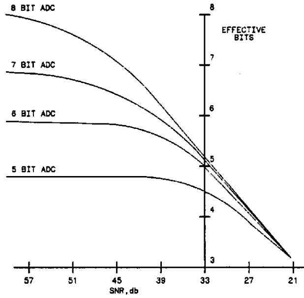
Figure A-1. Effective Bits Vs. Input Noise for Ideal A/D Converter.
