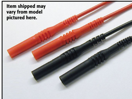
Model 8607 1kV Source Banana Cable Set: The 8607 cable set is made up of one red and one black high voltage test lead with fixed safety banana plug ends. The leads are 1 meter (3.3 ft) long and have a voltage rating of 1500V DC.
