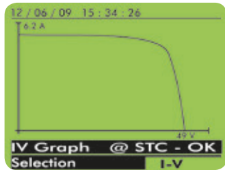
I-V curve
