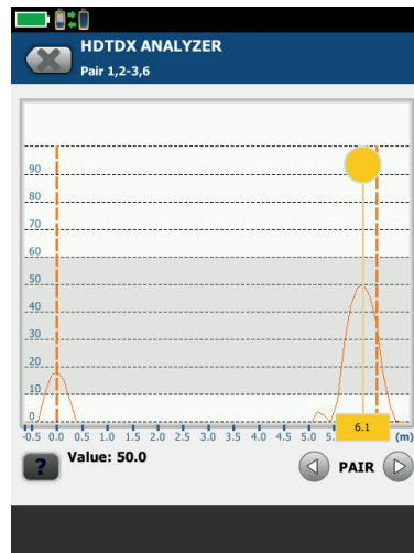
High Definition Time Domain Cross talk (HTDTCX) shows the far end connection is clearly the issue
