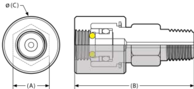
Neoprene 70 Replacement O-ring
