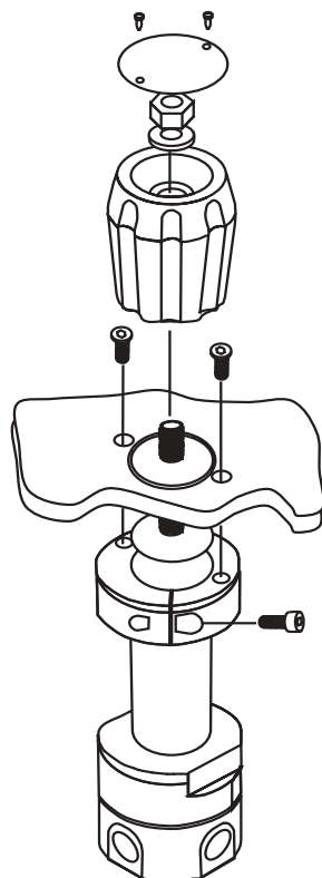
Figure 3-1. Standard Pneumatic Regulator (PN 65455)
