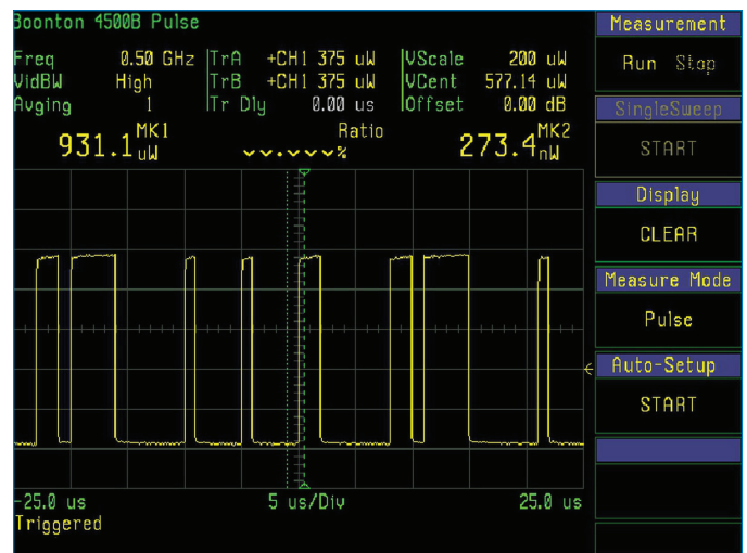
Fig 3: Example of a pulse train by using an external TTL compatible signal generator and modulated by the internal calibrator
