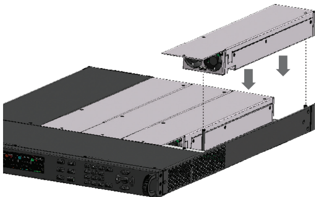
Module installation
