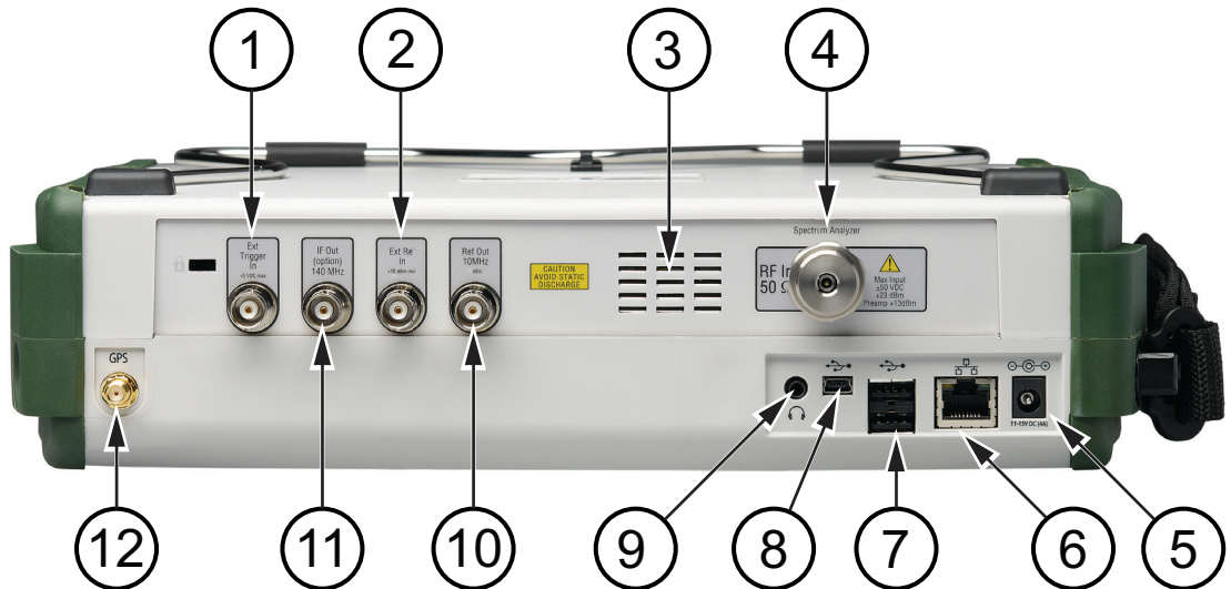
Figure 2-7. Test Panel Connectors for MS2720 Options 732, 743
