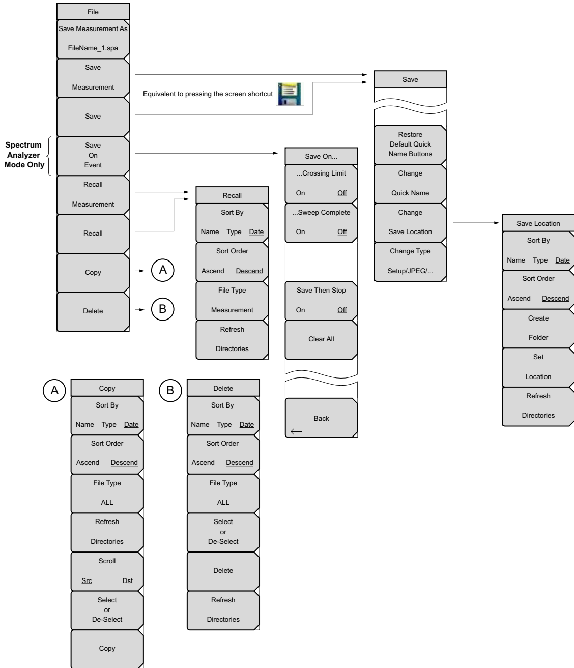
Figure 4-10. File Menu
