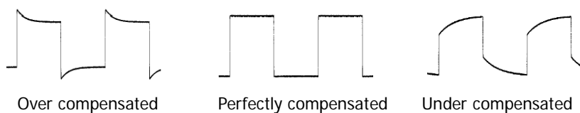
Figure 1-9 Probe Compensation
