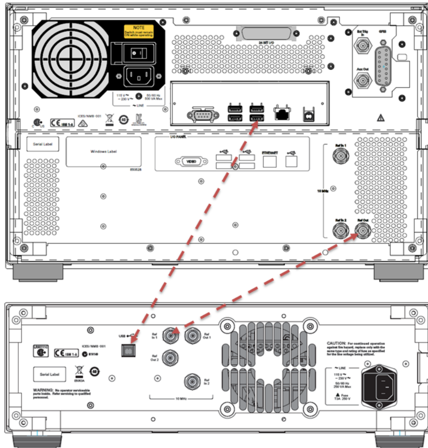
Figure 3-2 Connecting E5052B and E5053A (Rear Panel)
