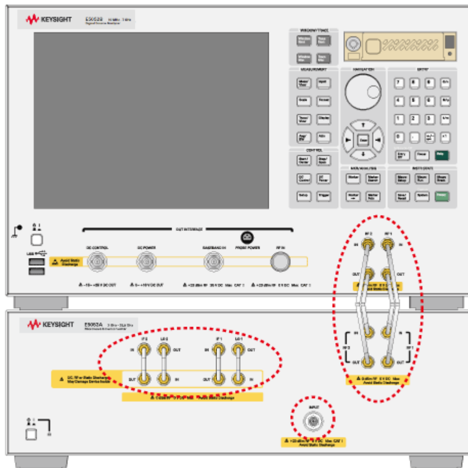
Figure 3-1 Connecting E5052B and E5053A (Front Panel)
