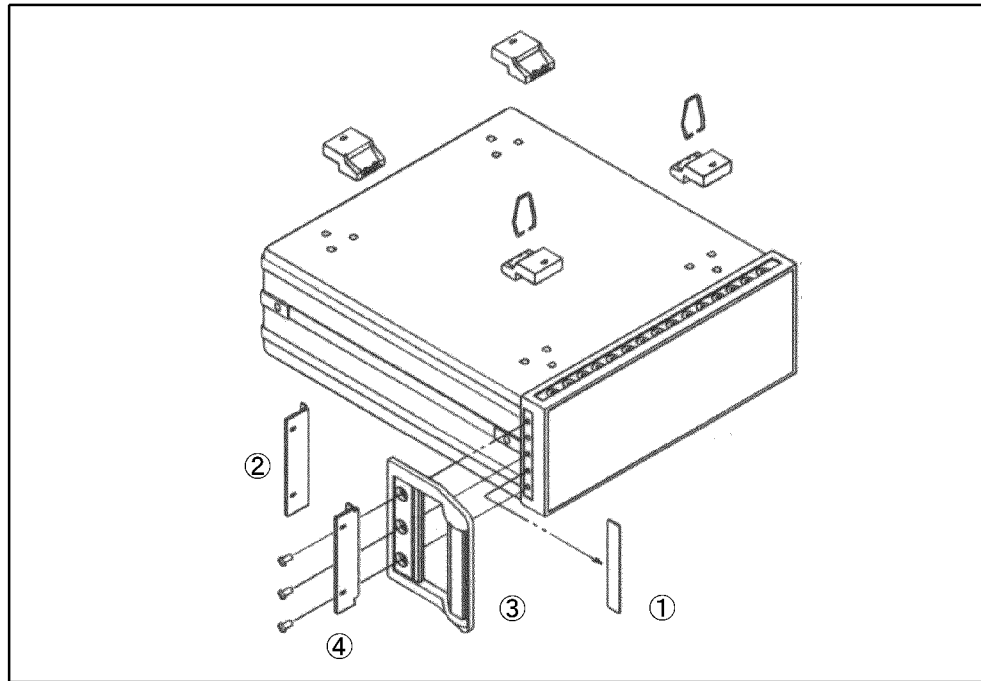
Mounting the handle/rackmount kit
