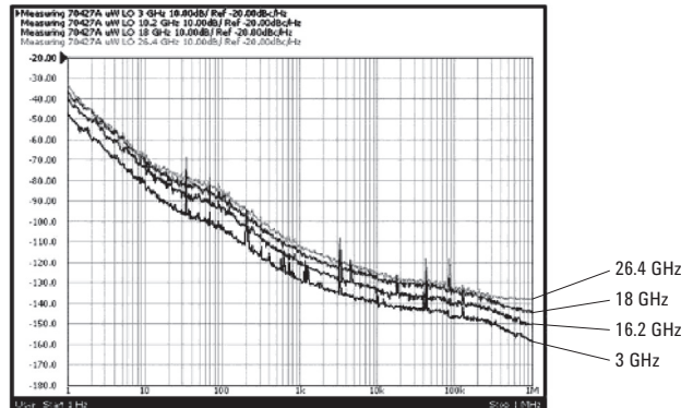
Figure 10-3. Measurement samples for the ultra-low noise N5507A LO
