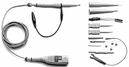
1165A 500 MHz passive probe
