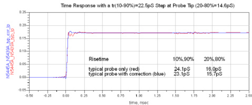
Time domain response plot with 1 mm span
