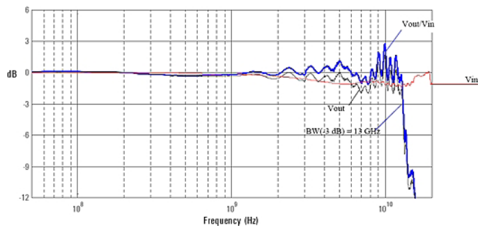
Frequency response of 1169B and N5381B with a 25 \Omega source
