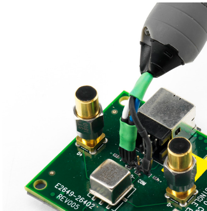
N2750A with N4822A socketed tip for application fixtures
