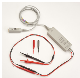
N2790A high voltage differential probe with N7013A extreme temperature extension kit
