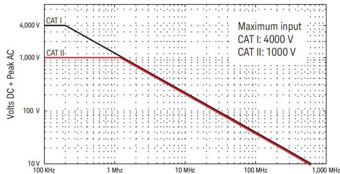
10076C derating curve
