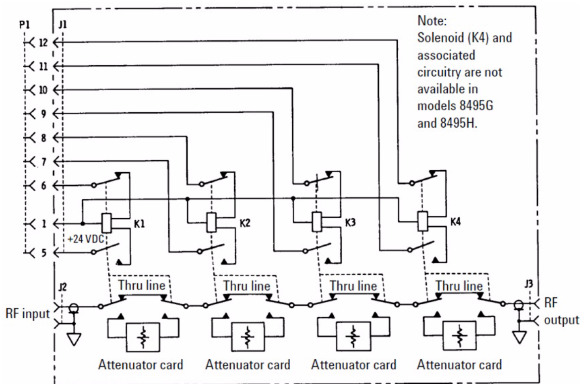
Figure 1 Typical Four-Section Attenuator Schematic Diagram
