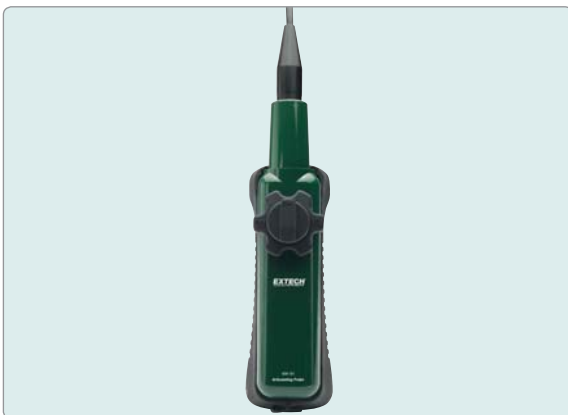
HDV-TX1, HDV-TX2 Wired handset with 6mm diameter semi-rigid articulated (320°) probe (1m, 2m versions)
