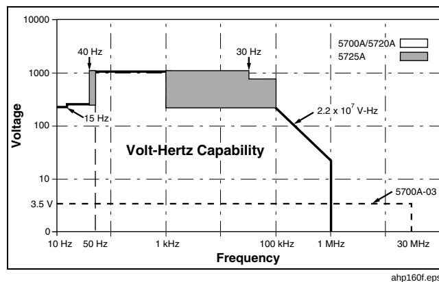
Figure 1-1. Volt-Hertz Capability
