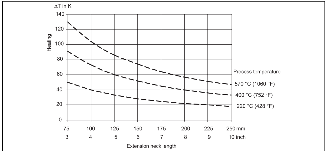
Heating of the field transmitter consequent to the process temperature. Temperature in the field transmitter = ambient temperature + \Delta T
