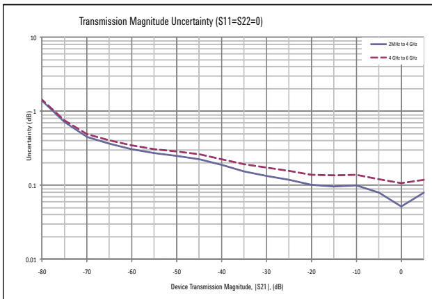
Figure 6: Transmission uncertainty
