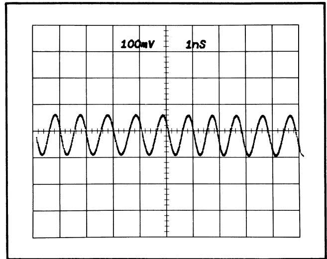
Fig. 2-3. 1 ns period sine wave display.
