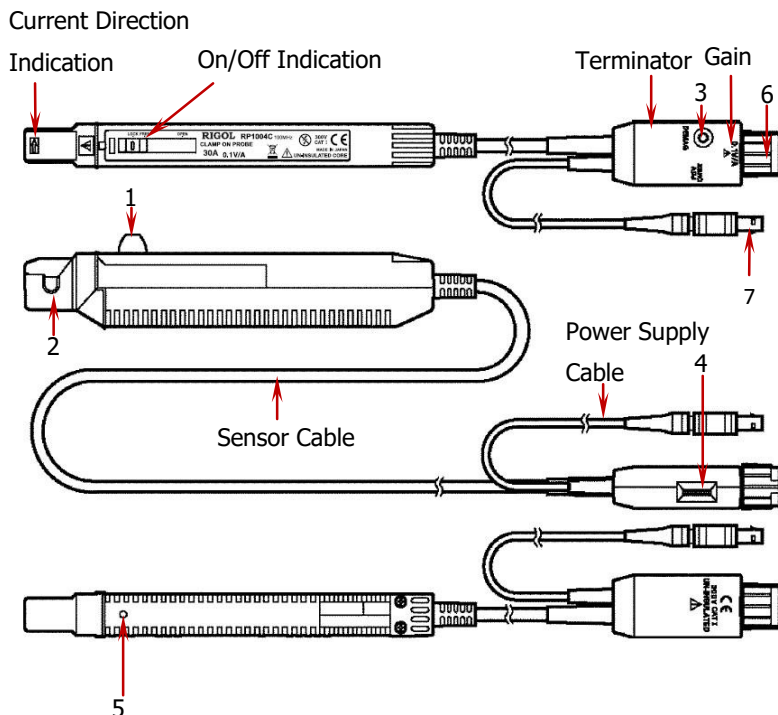
Figure 2 RP1004C Parts
