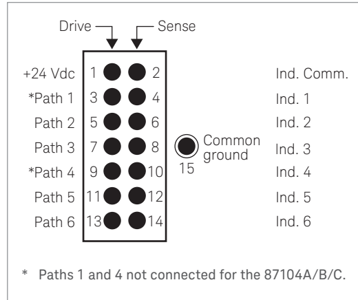
Figure 11. Drive connection diagrams with Option 100
