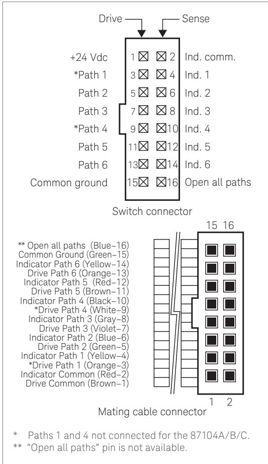
Figure 10. Drive connection diagrams with Option 161
